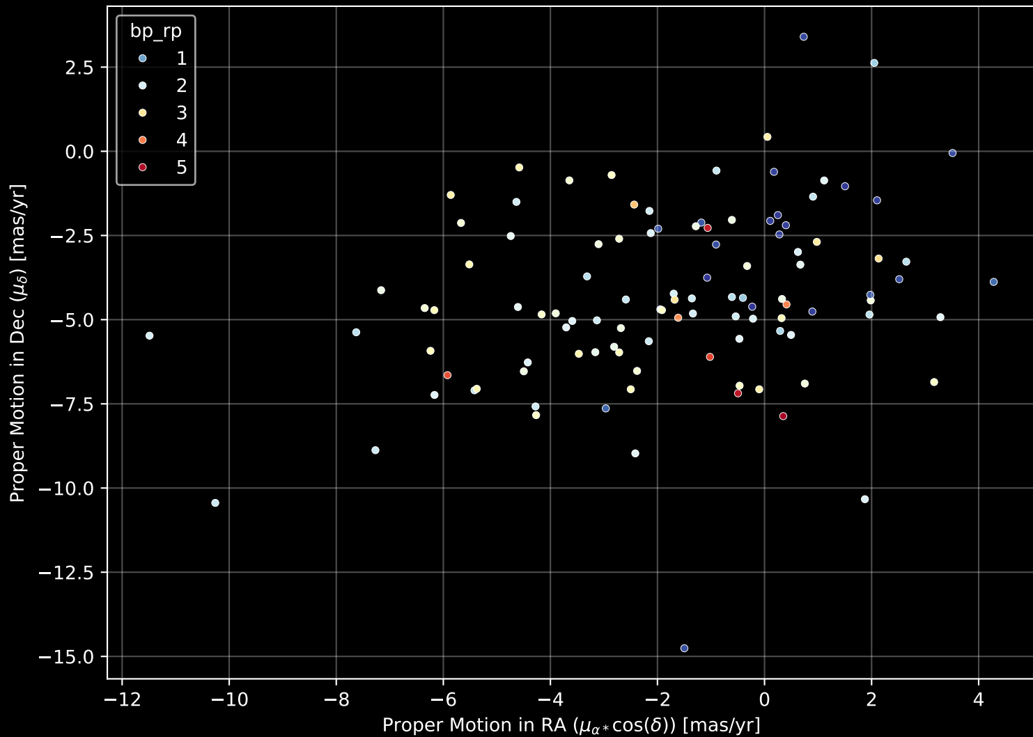
APOGEE DR17 Field: [003-05] Proper Motion Diagram (n= 108)
