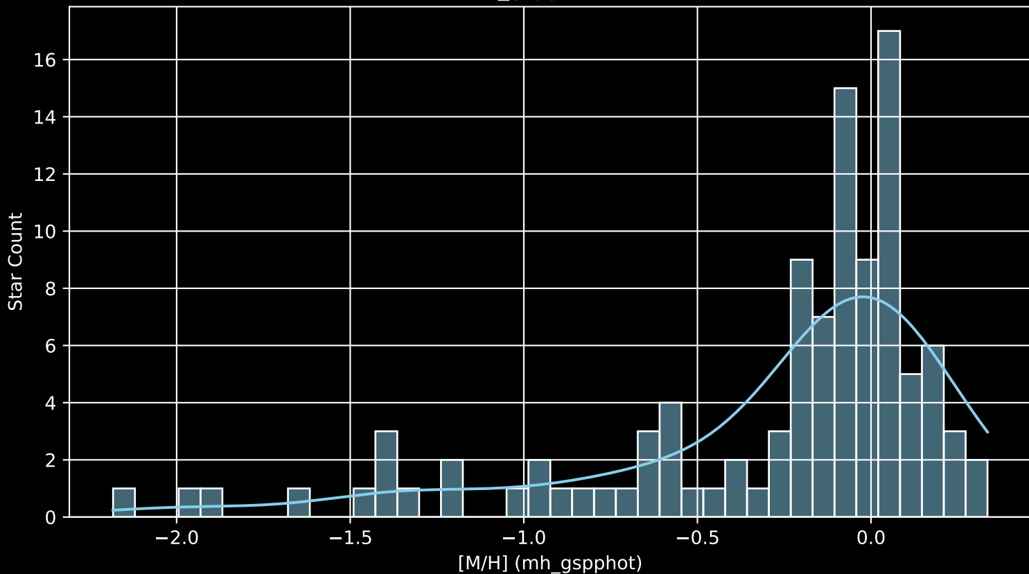
APOGEE DR17 Field: [003-05 [M/H] (mh_gspphot) (n= 106)
