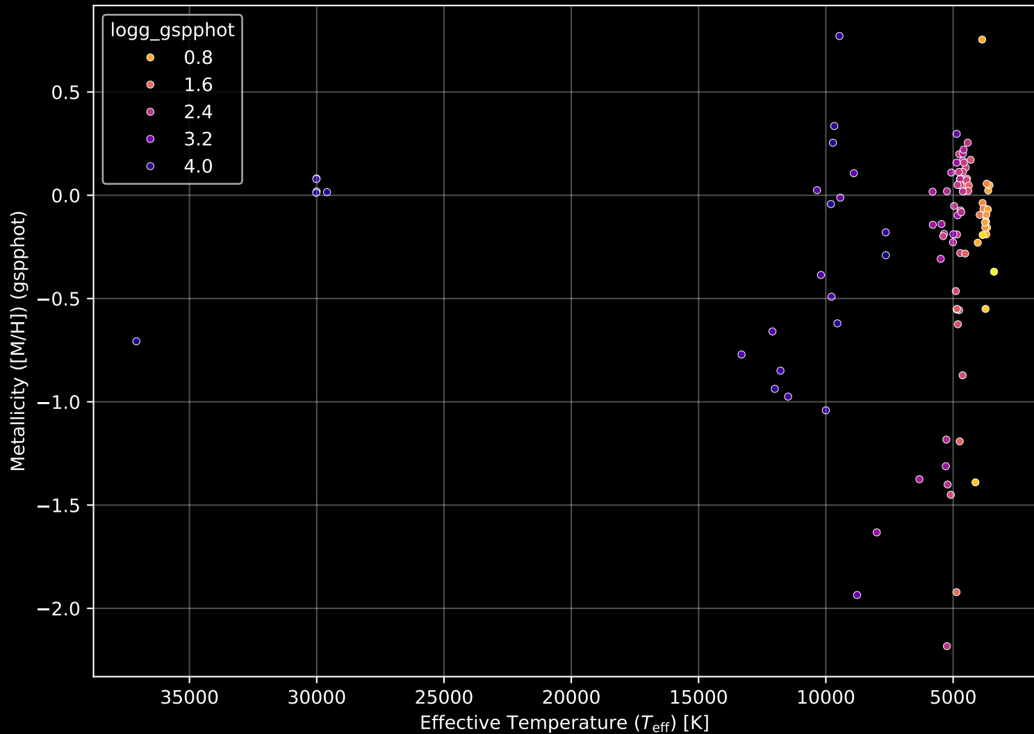
APOGEE DR17 Field: [003-05] Stellar Population Parameters (n= 108)
