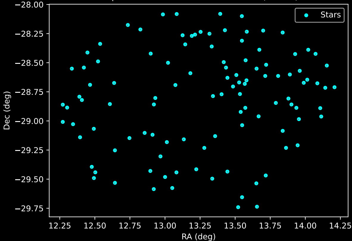
APOGEE DR17 Field: [003-05] Proper Motion Vectors for Gaia Star Field (n= 108)
