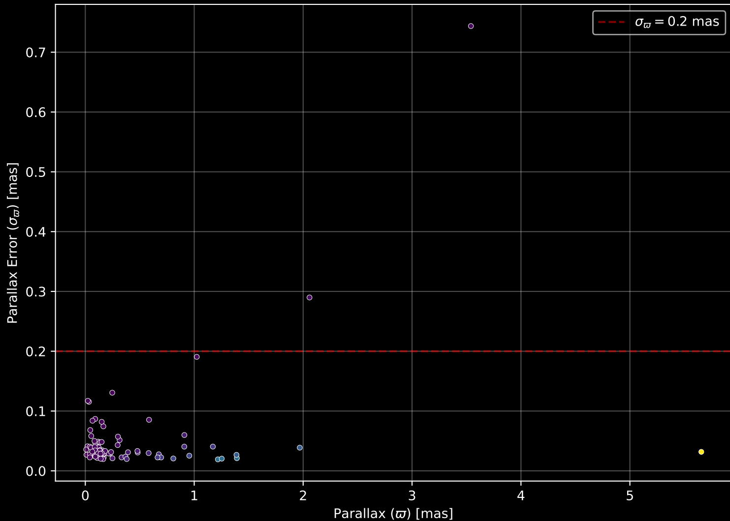
APOGEE DR17 Field: [003-05] Parallax Quality (n= 108)
