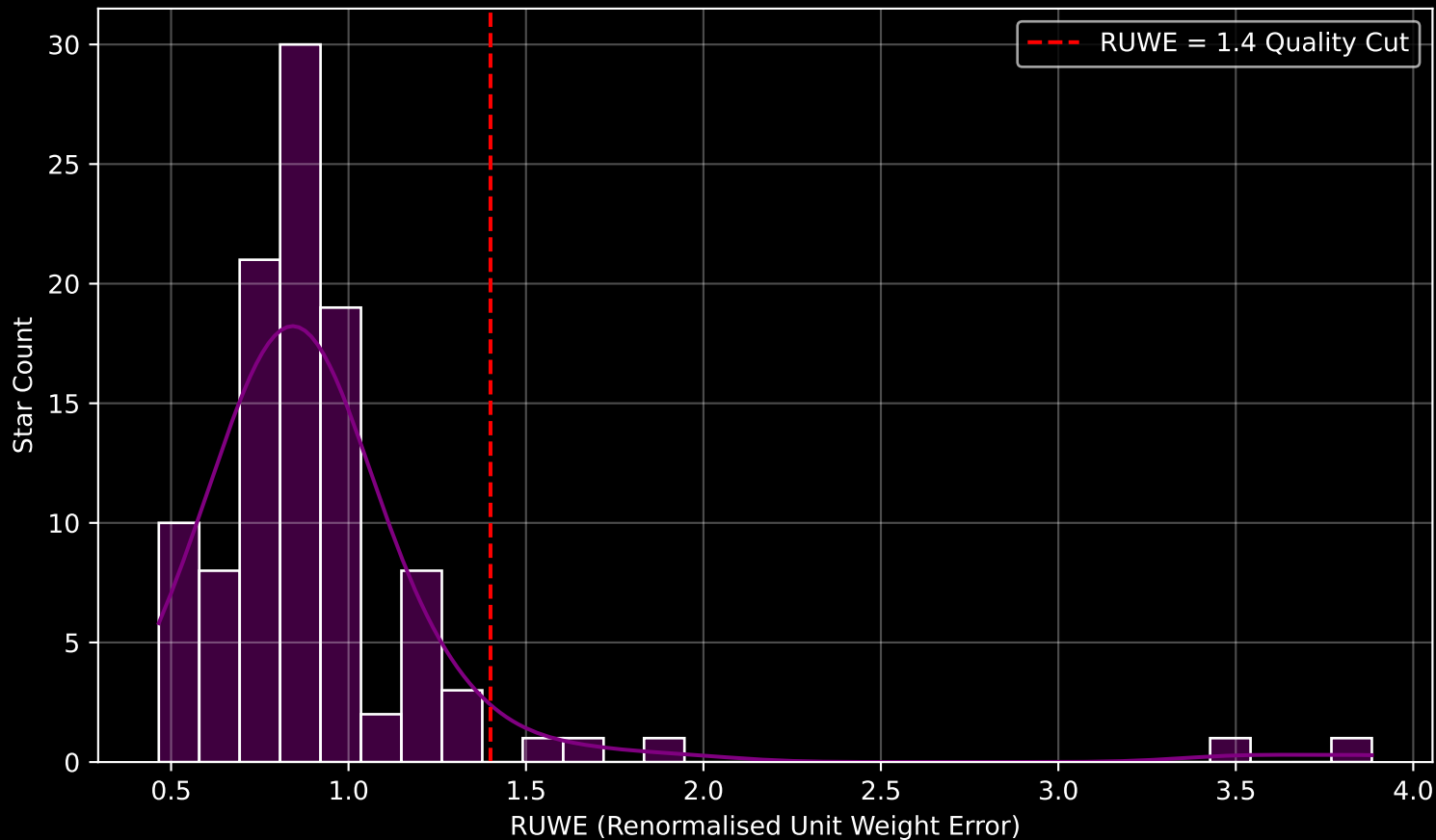
GAPOGEE DR17 Field [003-05] RUWE Distribution (n= 106)
