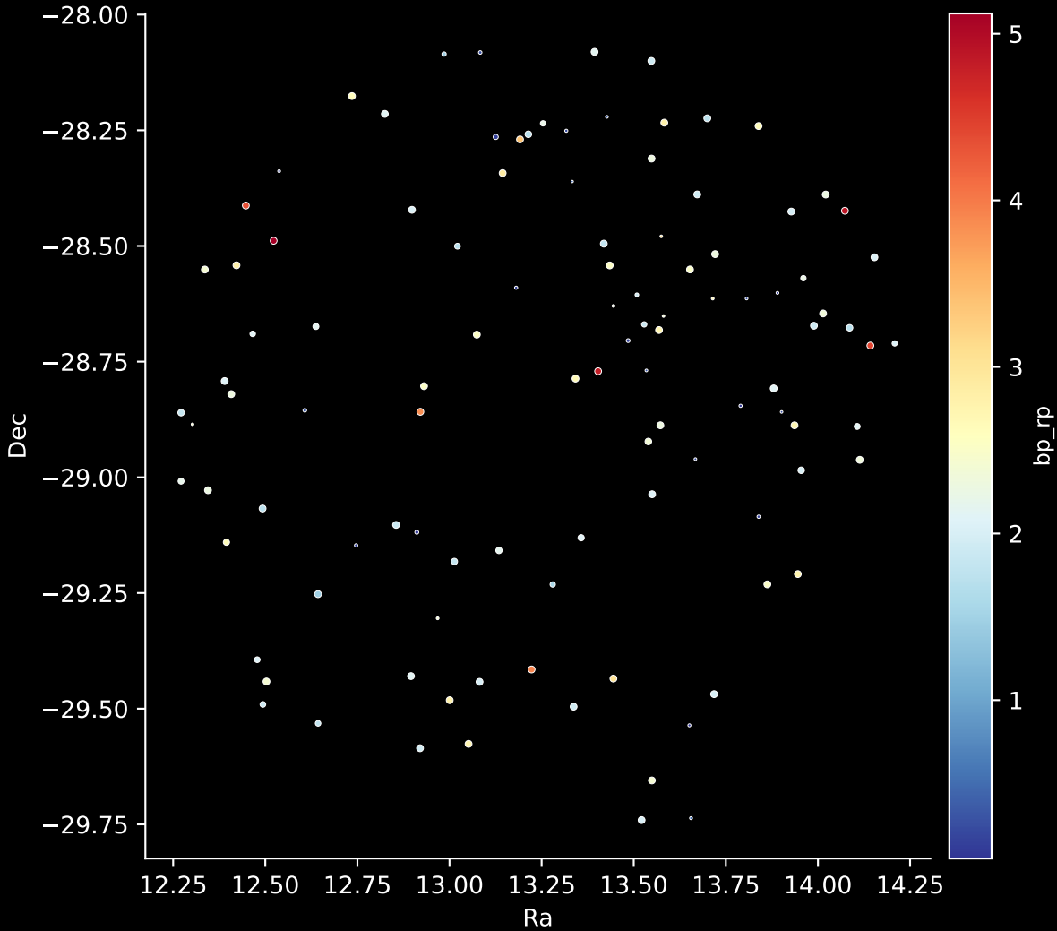
APOGEE DR17 Field: [003-05] Stars: 108
